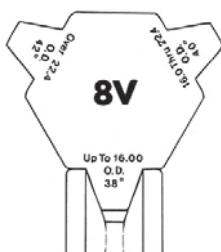
Sheave Groove Gauge
